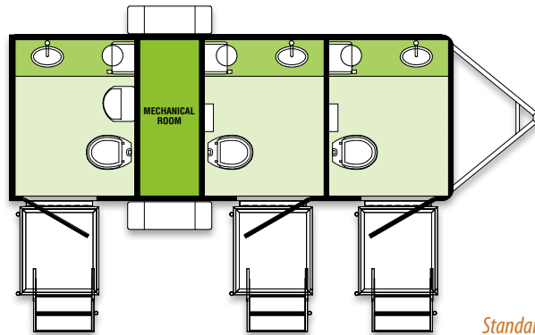
Standard Floorplan
