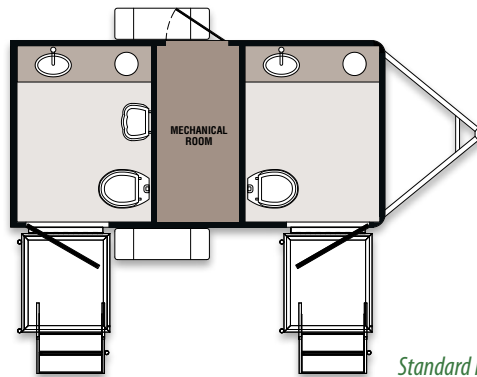
Standard Floorplan
